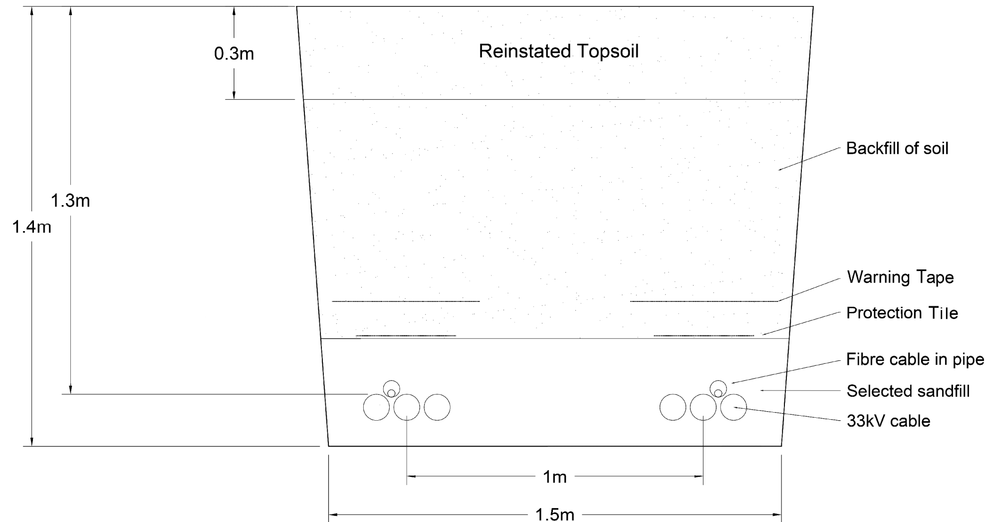
Typical Cable Trench
