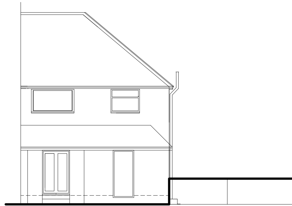
FRONT ELEVATION
