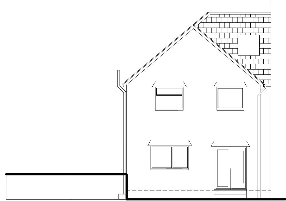
REAR ELEVATION
