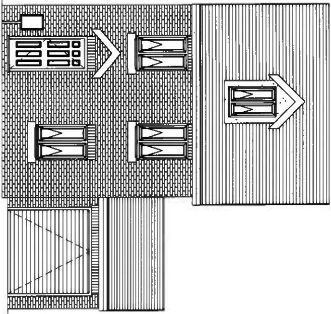
1 Proposed Front Elevation 1 : 100
