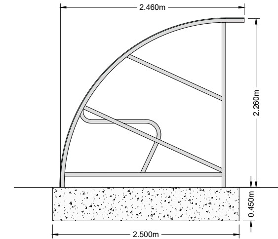
SOUTHERN ELEVATION
