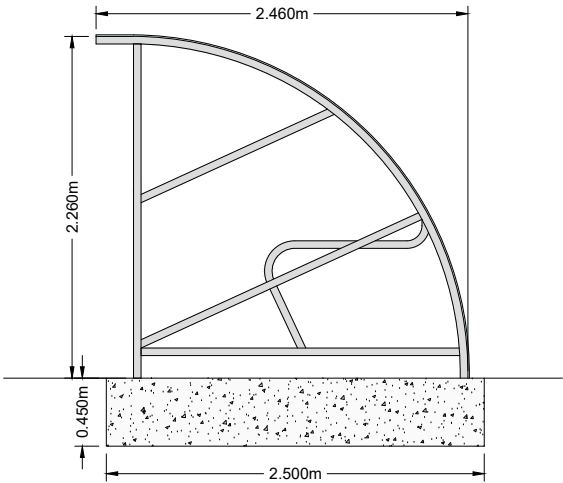
NORTHERN ELEVATION
