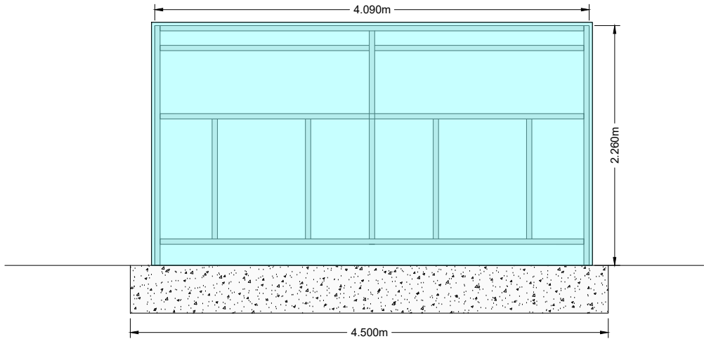
EASTERN ELEVATION
