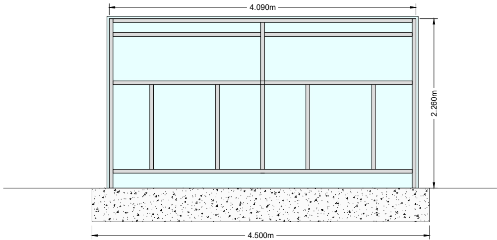
WESTERN ELEVATION
