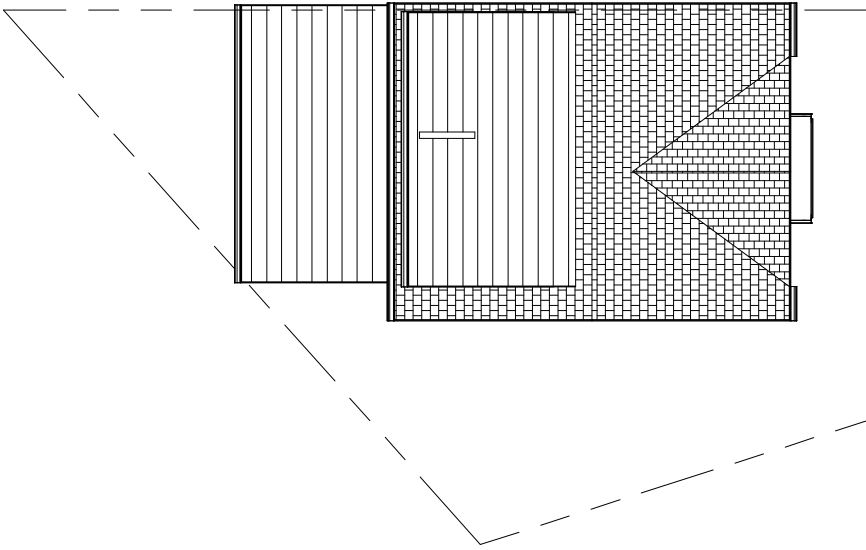
2 Proposed Site 1 : 100
