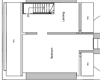
⑧ Existing Second Floor 1 : 100
