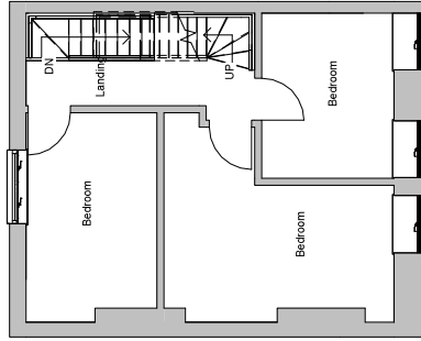
⑦ Existing First Floor 1 : 100
