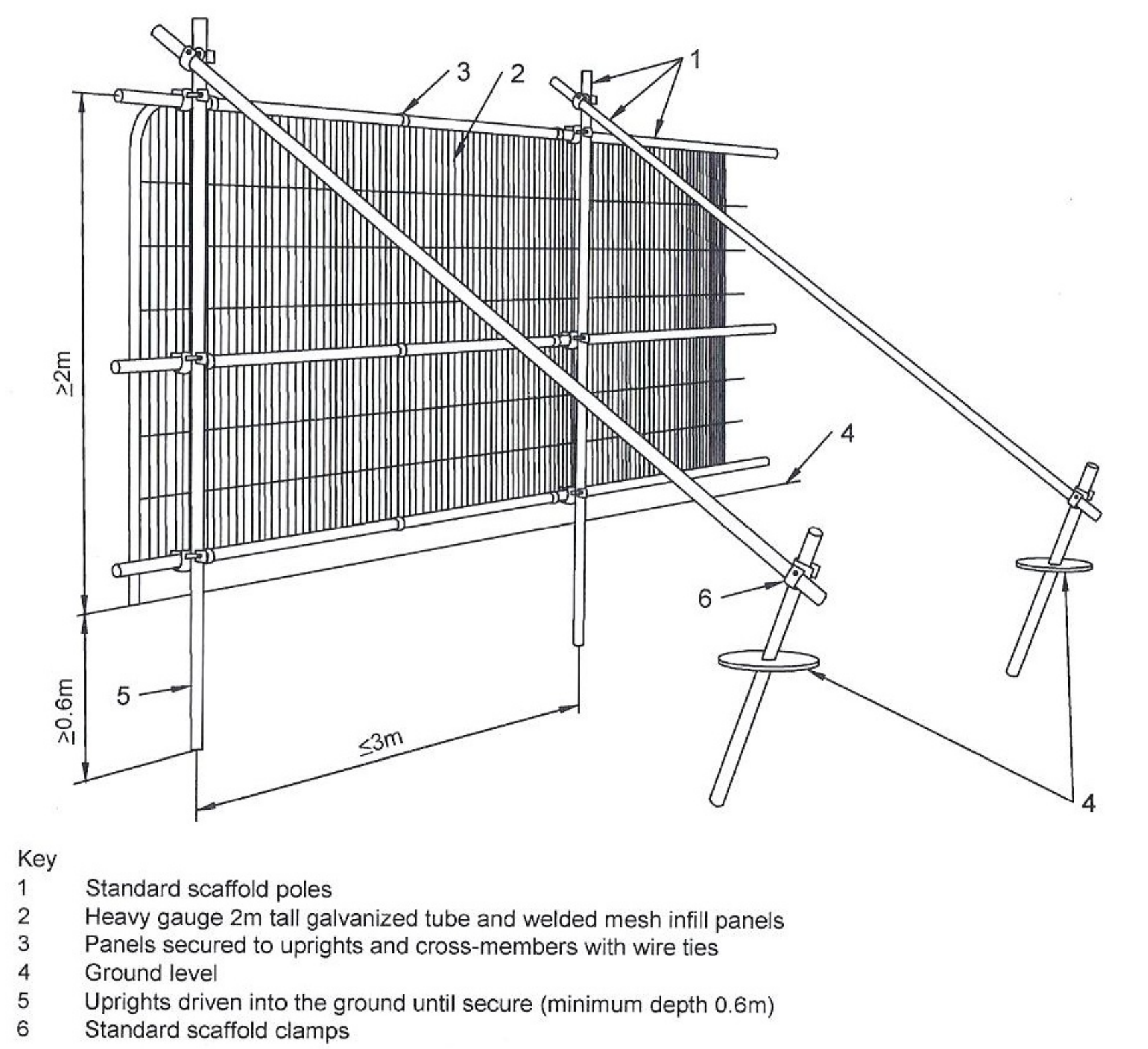
Figure 2 Default specification for protective barrier
