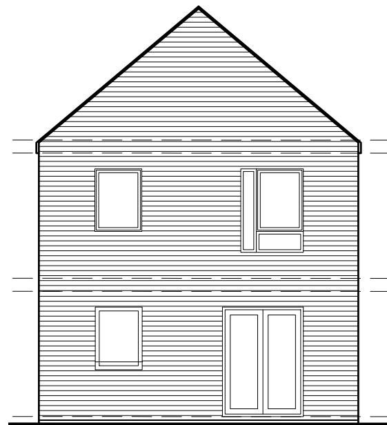
REAR ELEVATION
