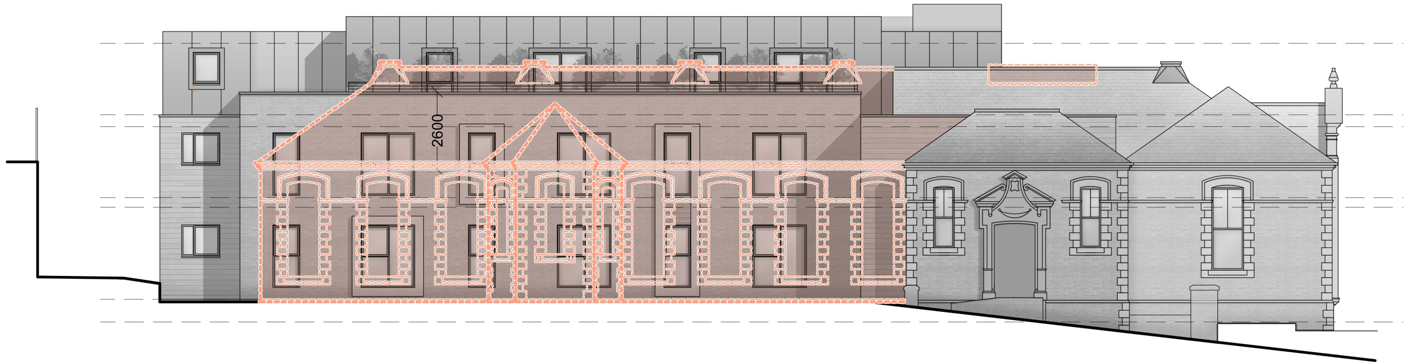
Gwaelodygarth (West) Elevation - Demolitions
