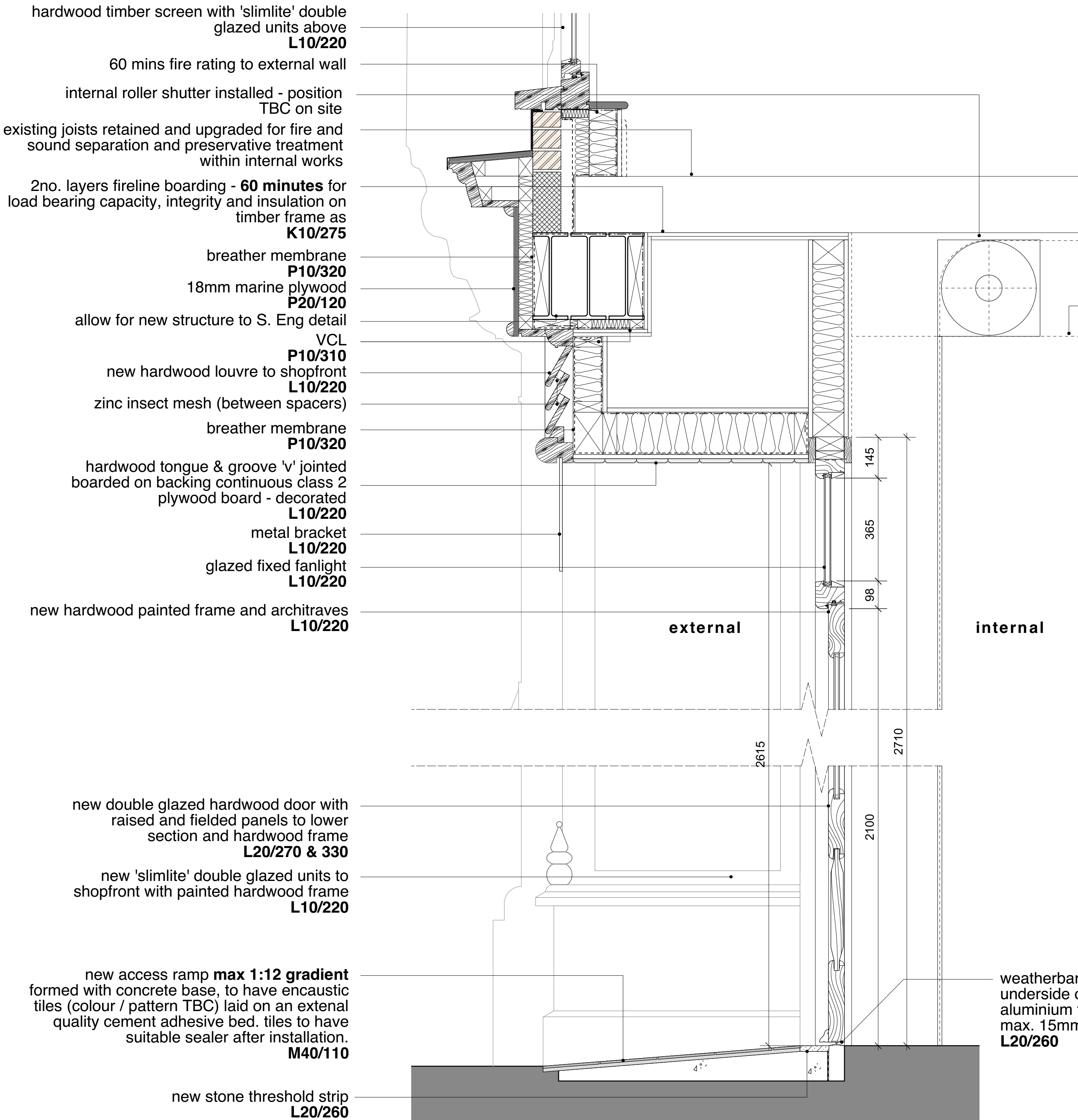
01 new timber shopfront section detail (through door)
