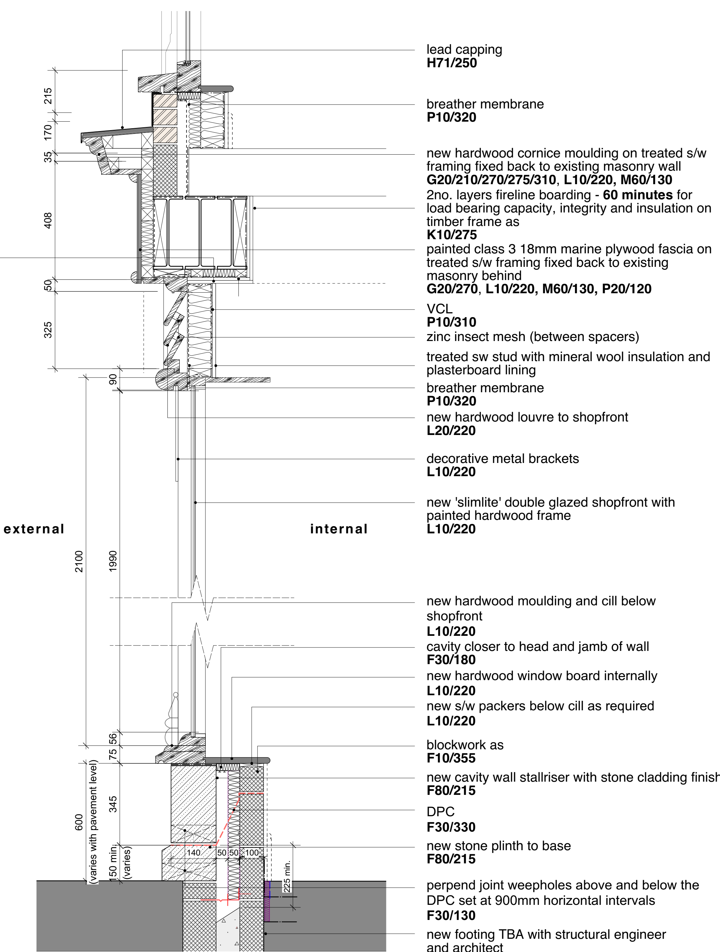
02 new timber shopfront section detail (through glazing)
