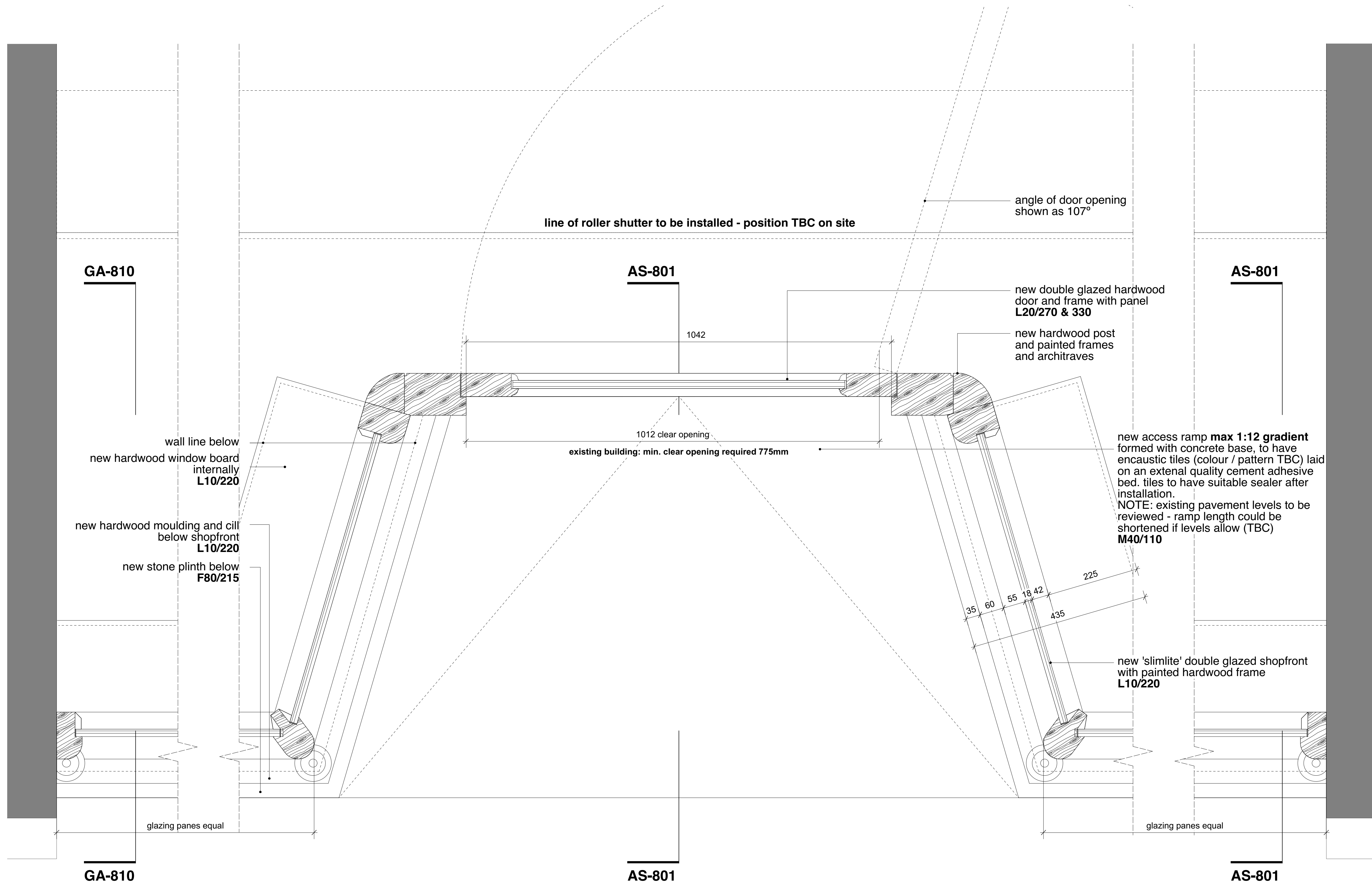
01 shopfront plan detail
