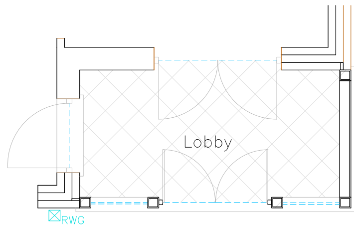
Proposed Extension Floor Plan 1:50
