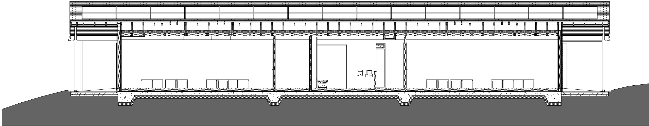
Proposed - Building Section 1
