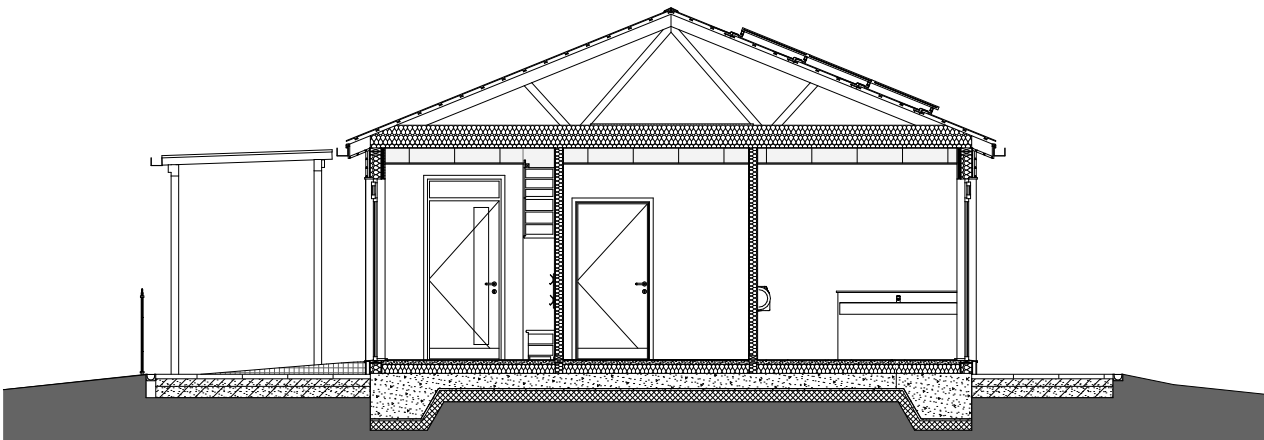
Proposed - Building Section 4
