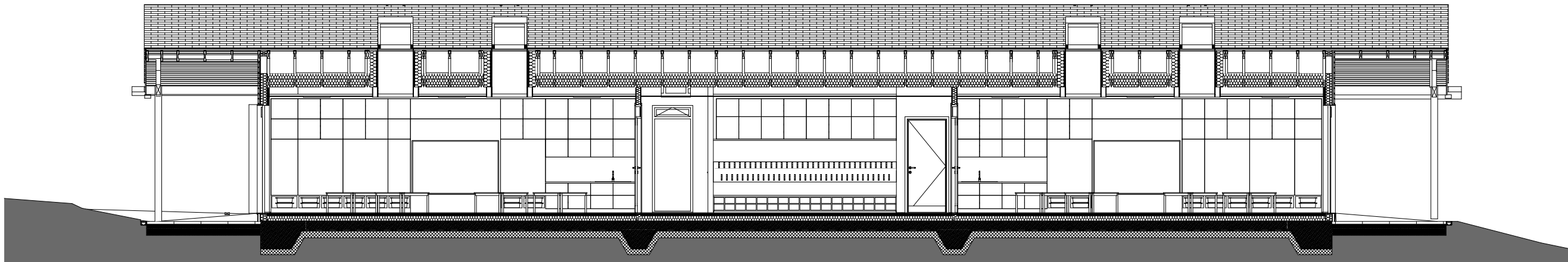
Proposed - Building Section 2
