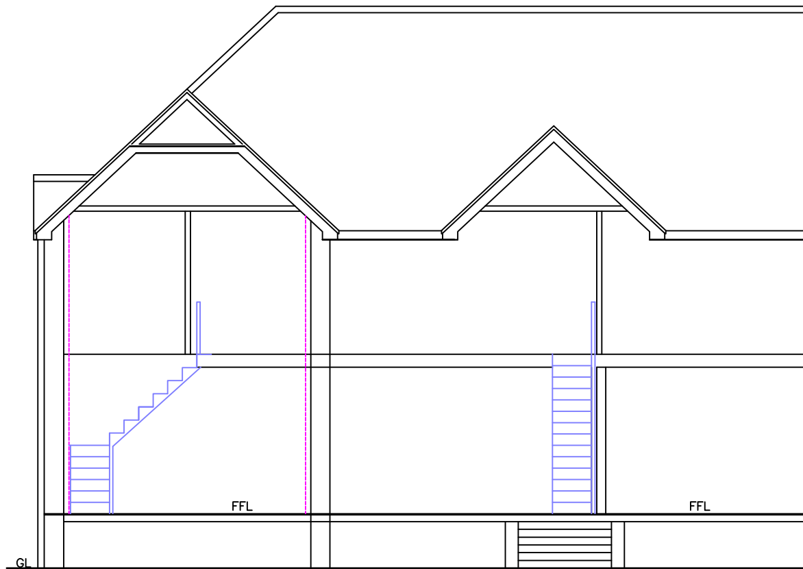
Proposed Section 1:100
