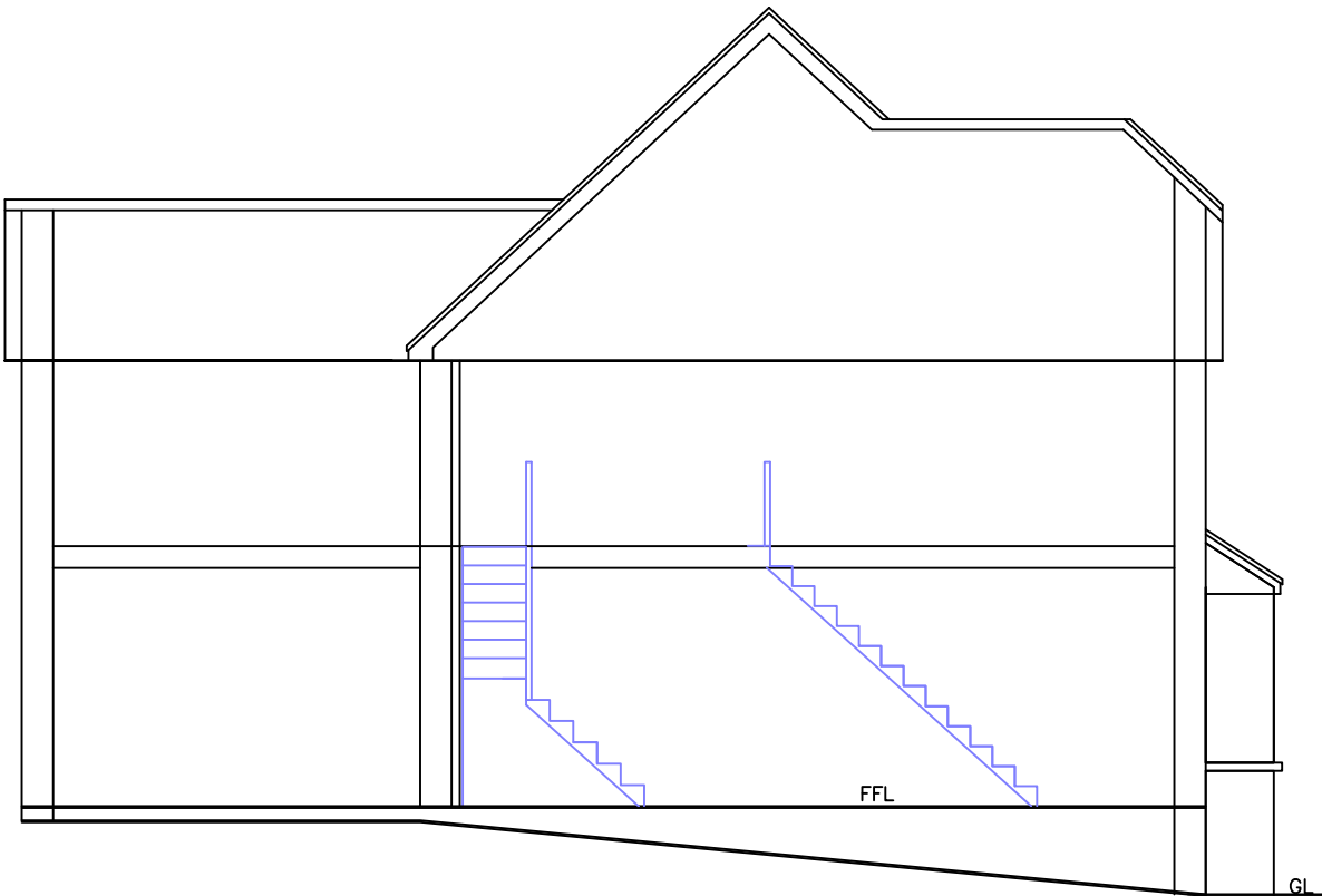
Proposed Section 1:100
