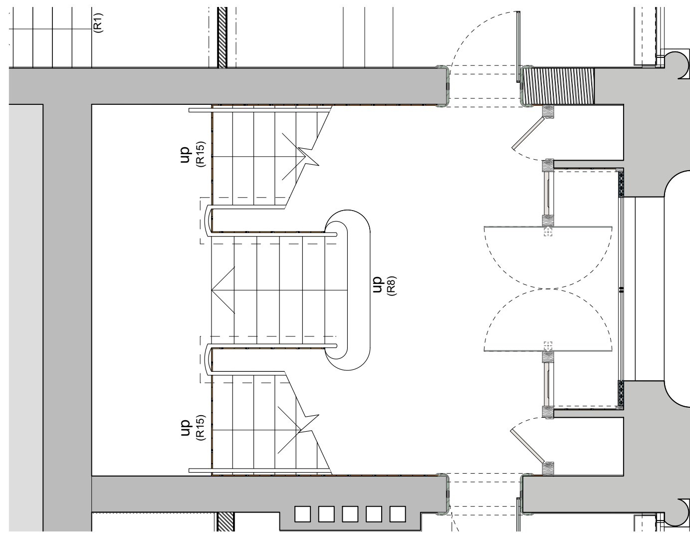
A 550.1 STAIRHALL PLAN SCALE 1:50 @ A1, 1:100 @ A3
