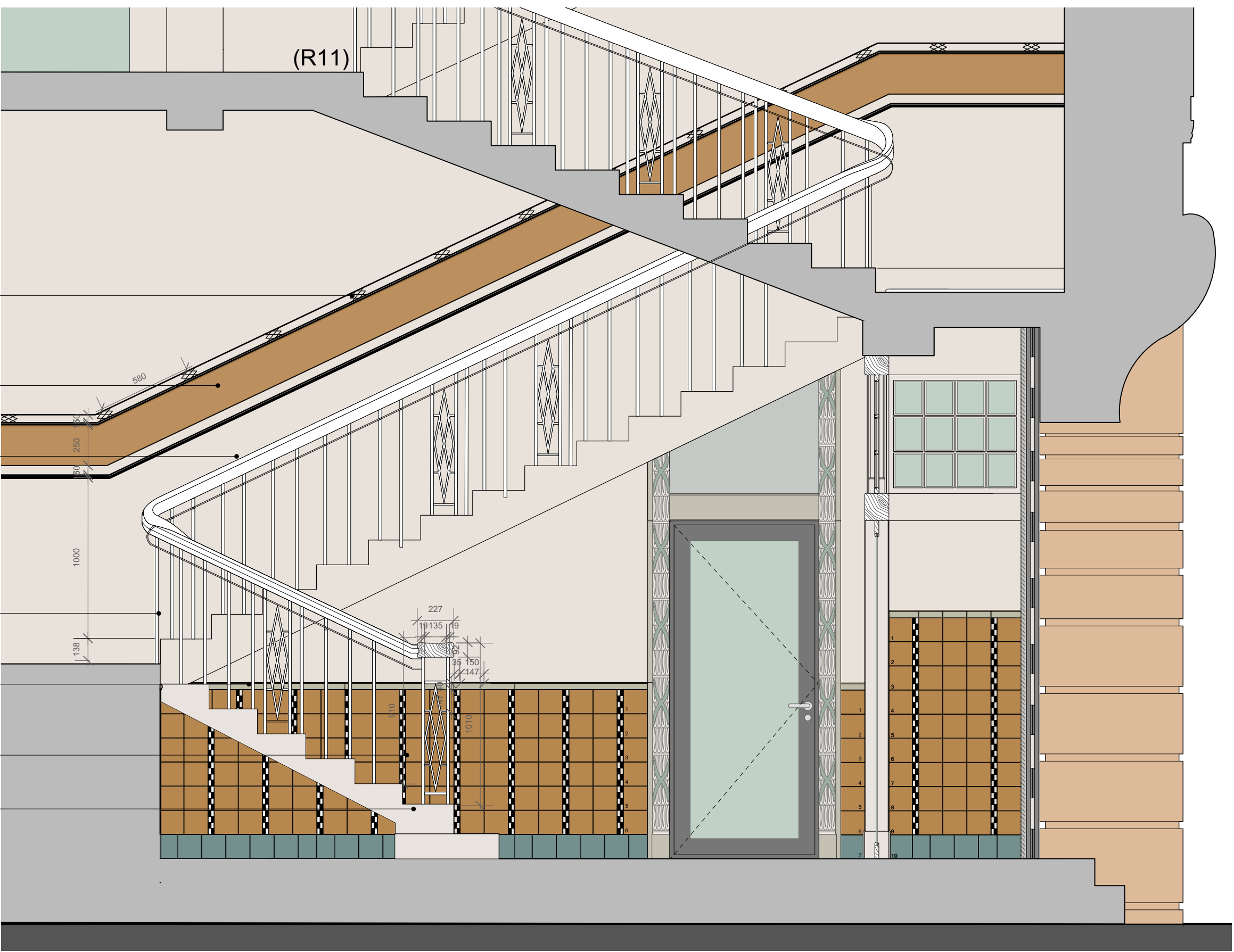
A 550.4 DETAIL SECTION SCALE 1:25 @ A1, 1:50 @ A3
