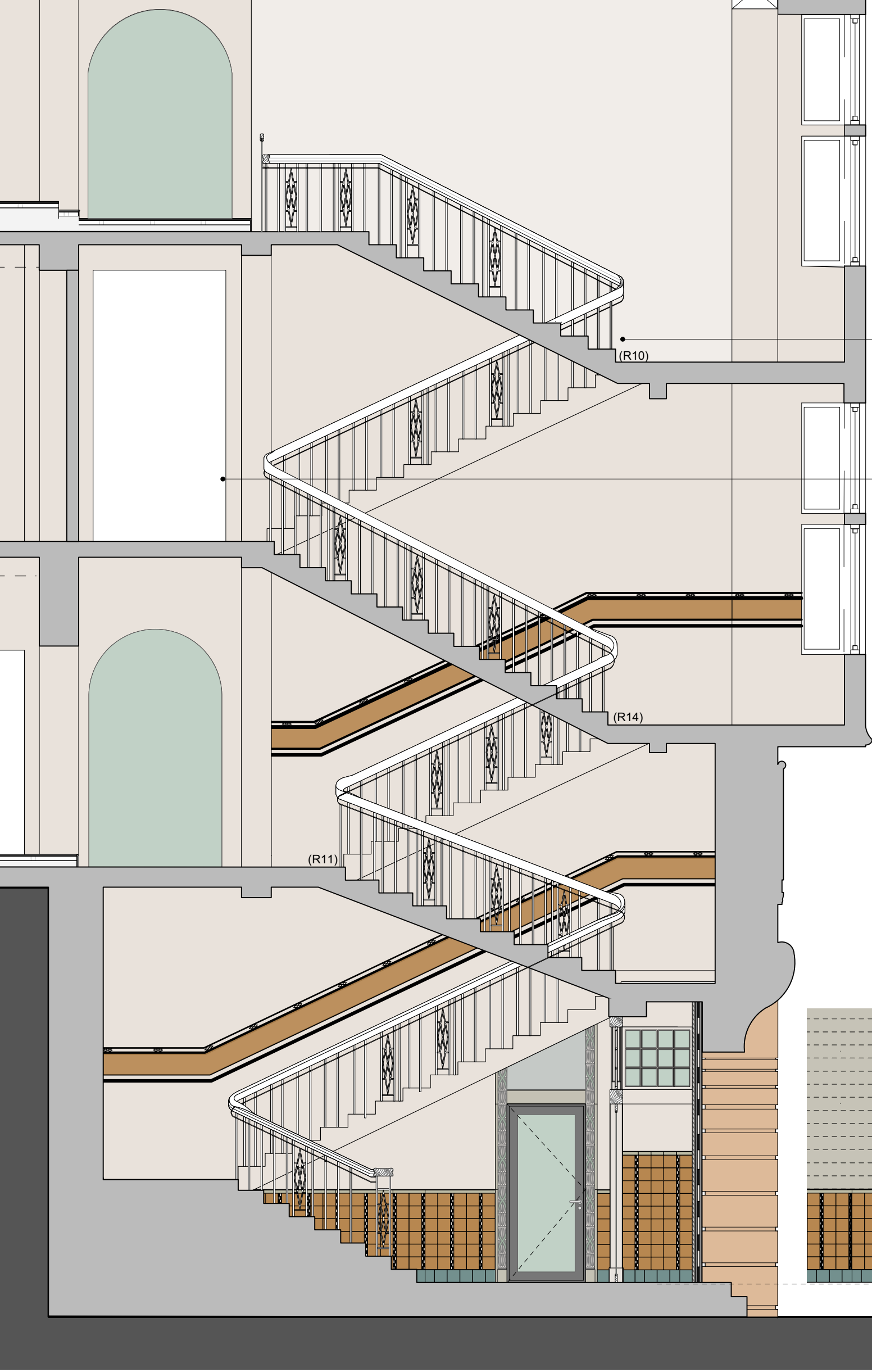
A 550.2 STAIRHALL SECTION SCALE 1:50 @ A1, 1:100 @ A3
