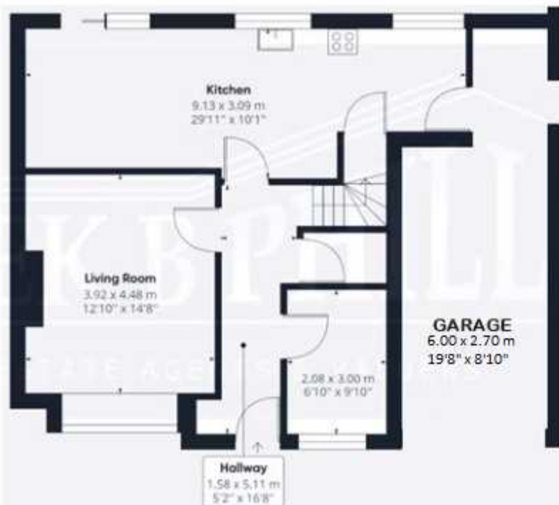
Floor 0 Building 1
