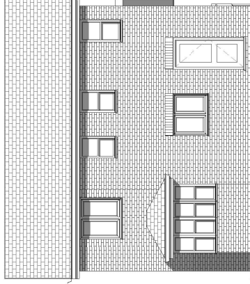
4 Existing Rear Elevation 1 : 100
