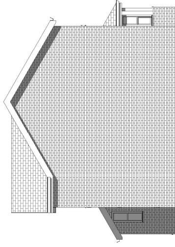
6 Existing Side 2 Elevation 1 : 100
