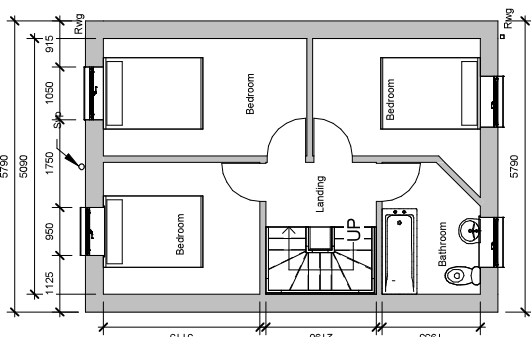
2 First Floor 1 : 100
