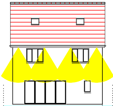
REAR ELEVATION
