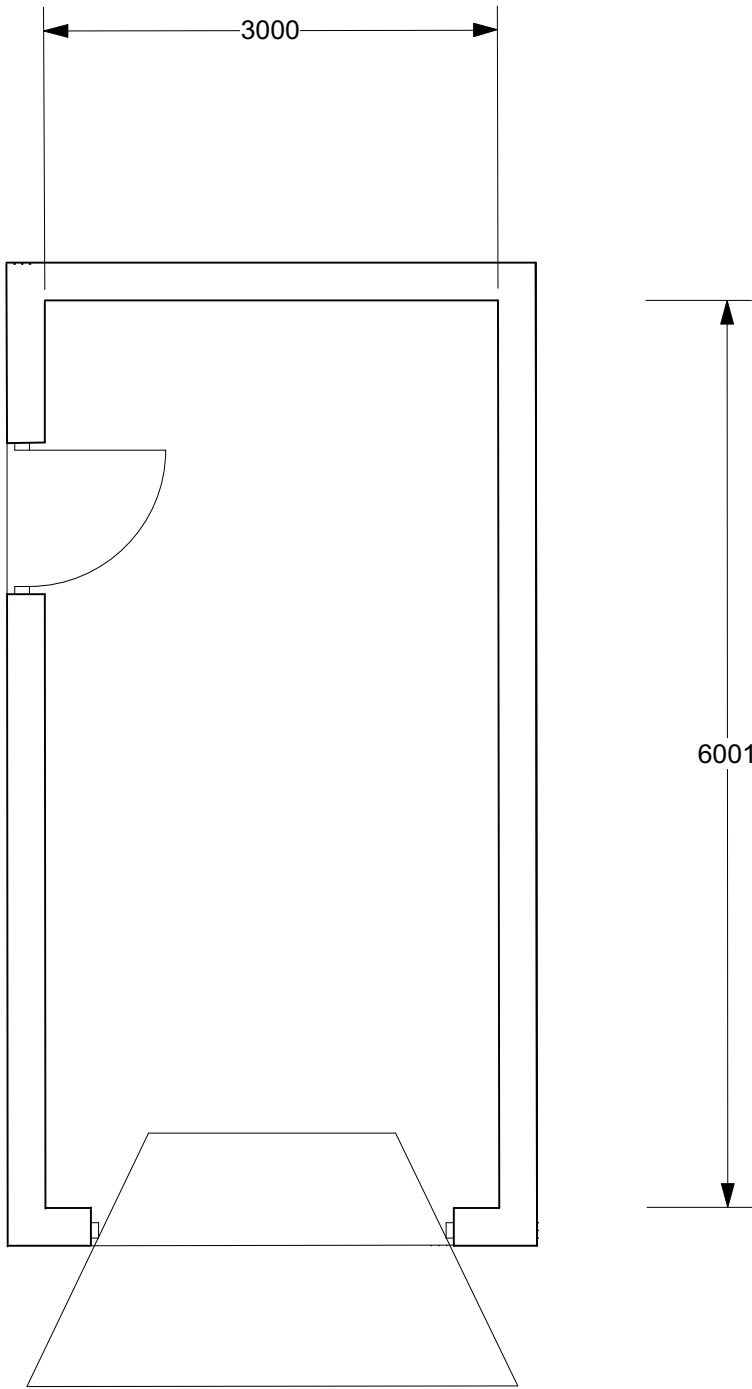
floor plan
