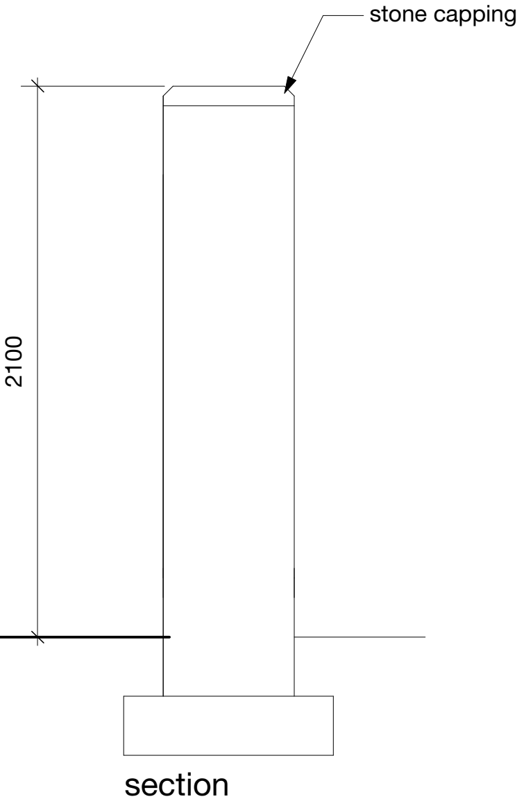
DETAILS OF FRONT GARDEN WALL
