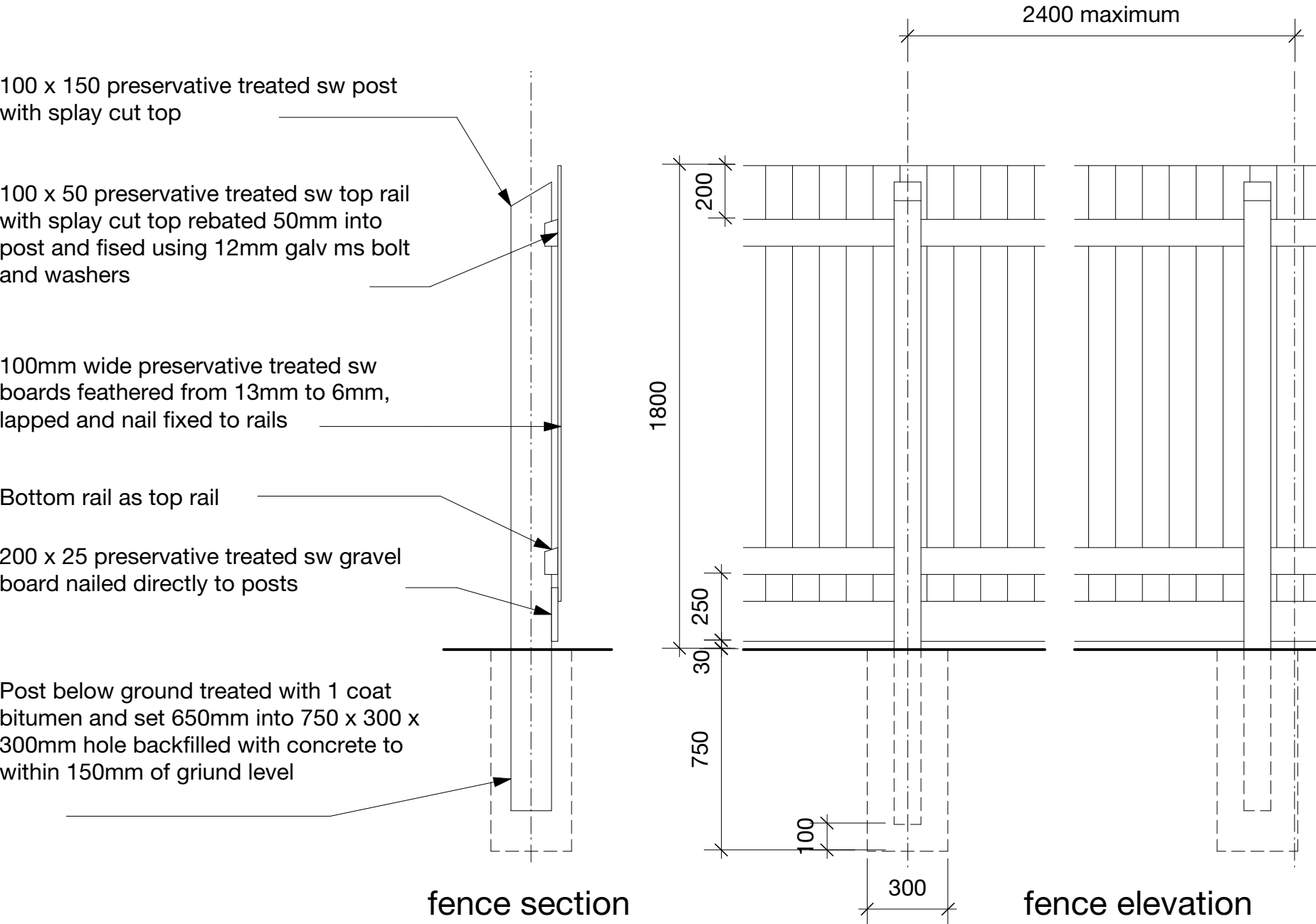
DETAILS OF FENCE G AND GATE H (1:20)
