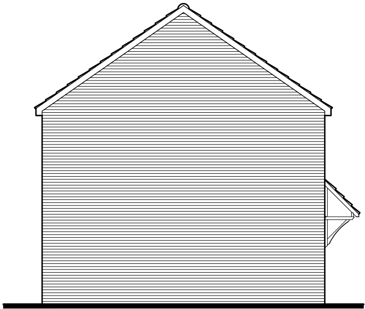
Side Elevation
