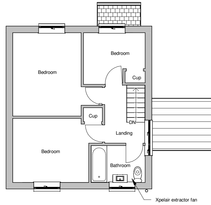
2 Existing First Floor 1 : 100
