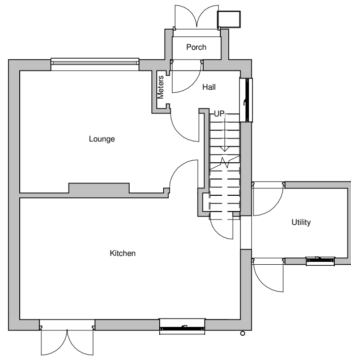
1 Existing Ground Floor 1 : 100
