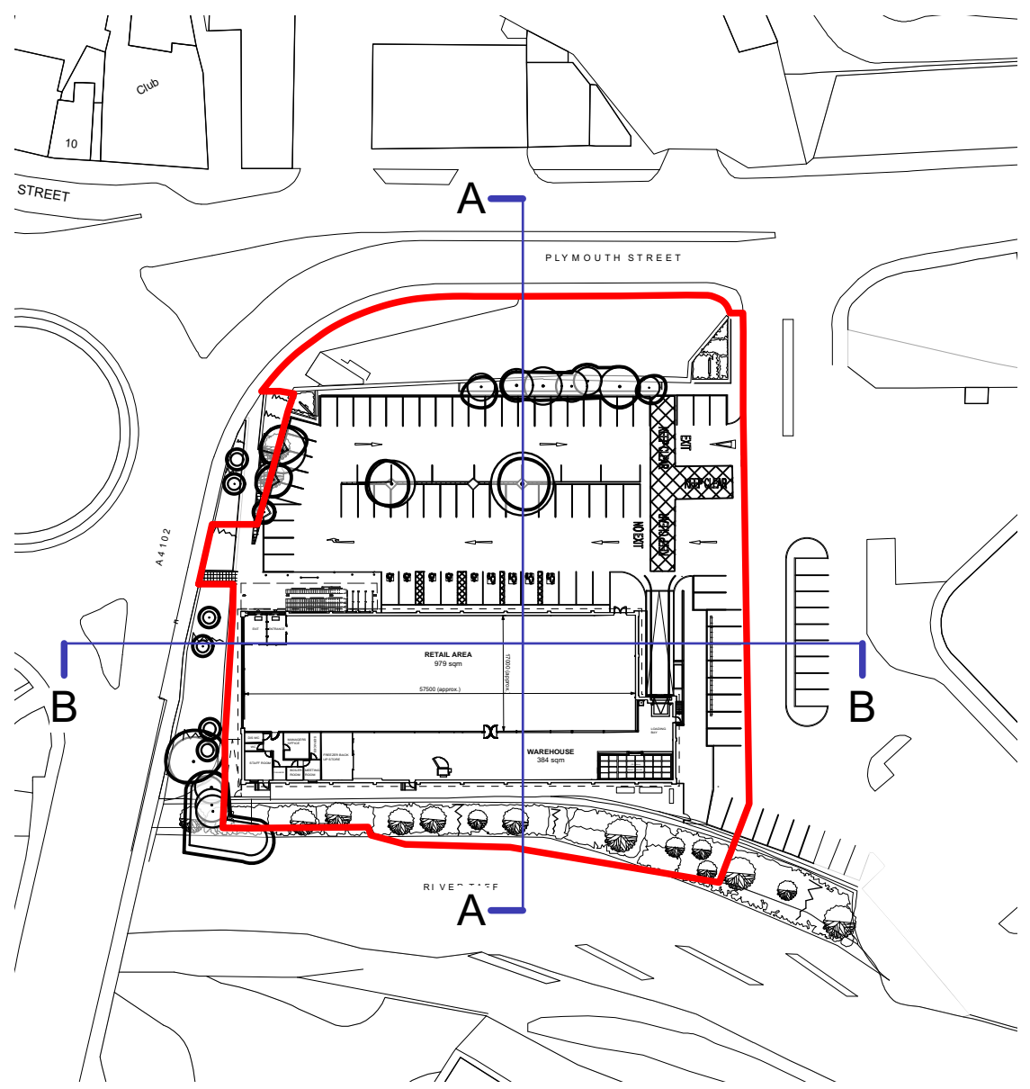
EXISTING SITE LOCATION PLAN
