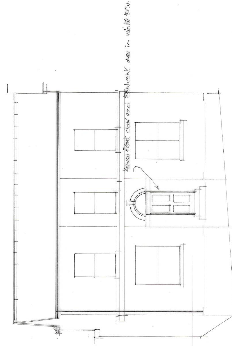
Proposed Front Elevation - south
