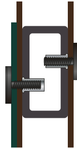
Box Section Internal Ladder Frame
