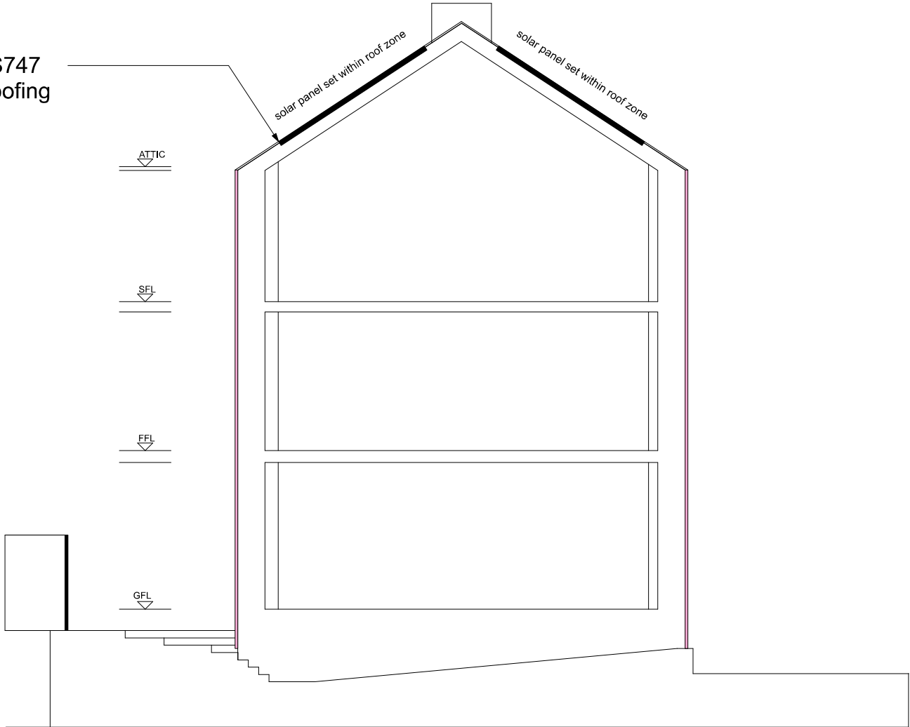
SECTION
