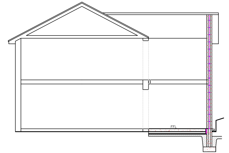
Proposed Section 1:100
