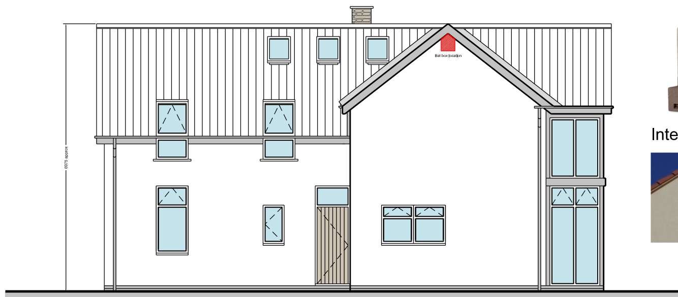
Rear Elevation - 1:100 @ A3
