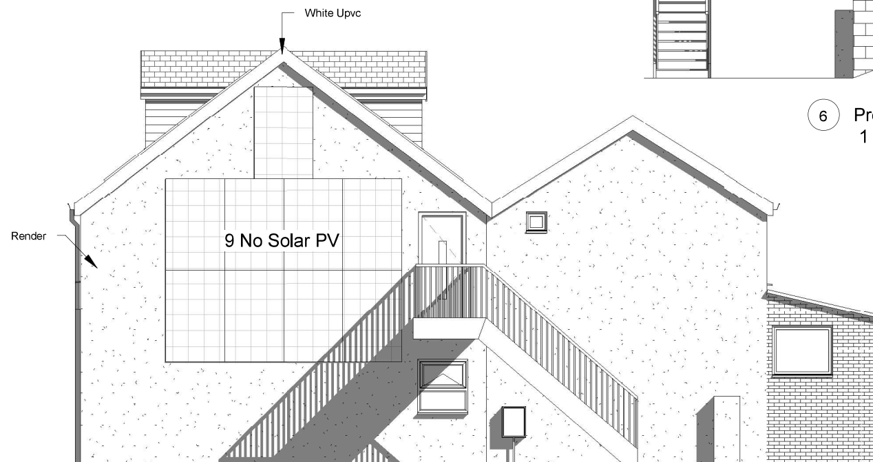
5 Proposed Side Elevation 1 : 100
