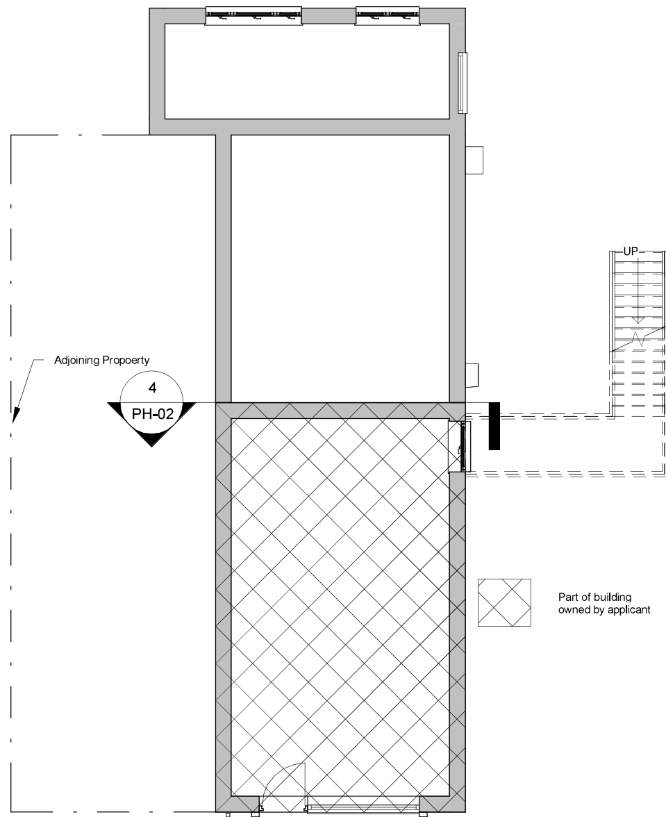
1 Proposed Ground Floor 1 : 100
