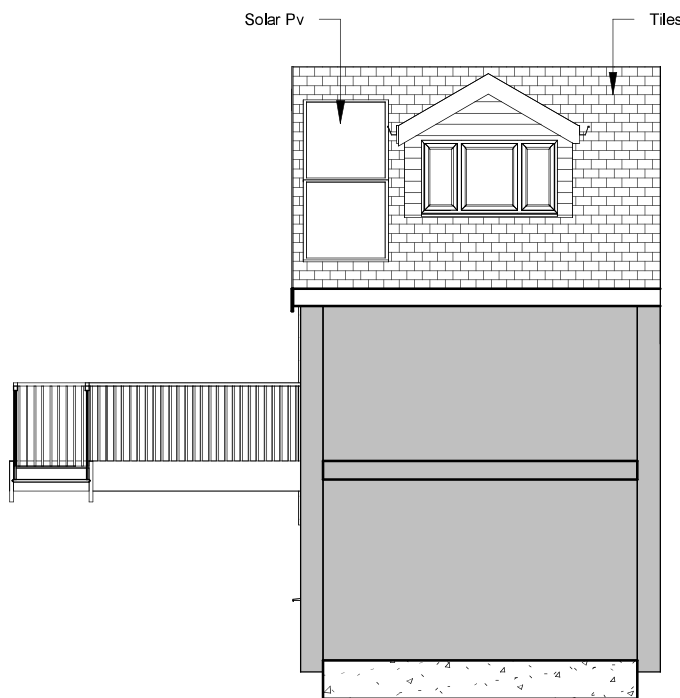
4 Proposed Rear Roof Section 1 : 100
