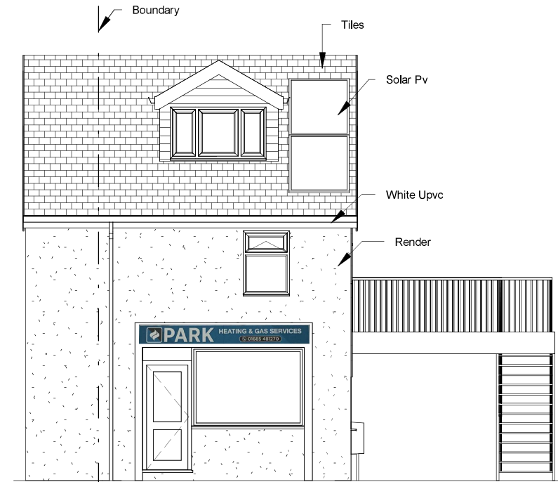
3 Proposed Front Elevation 1 : 100
