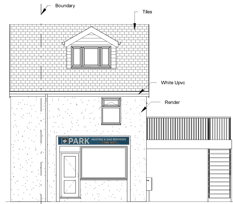
3 Existing Front Elevation 1 : 100
