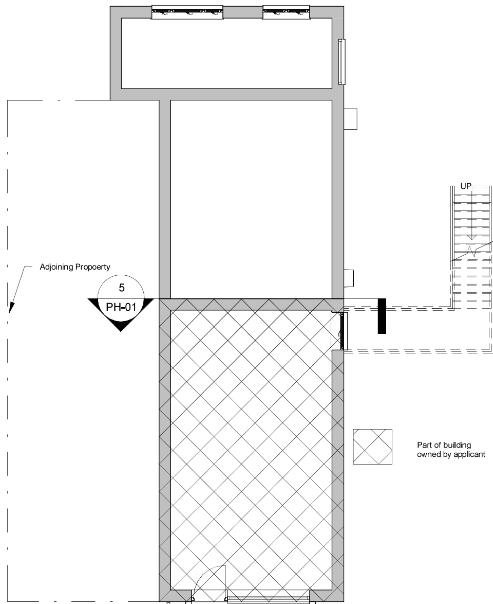
1 Existing Ground Floor 1 : 100
