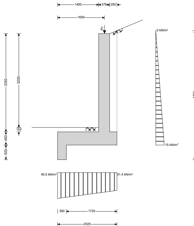
General arrangement
