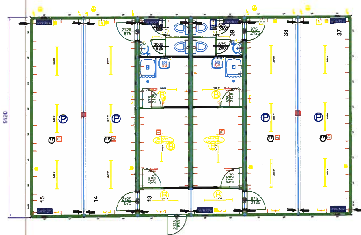
FLOOR PLAN
