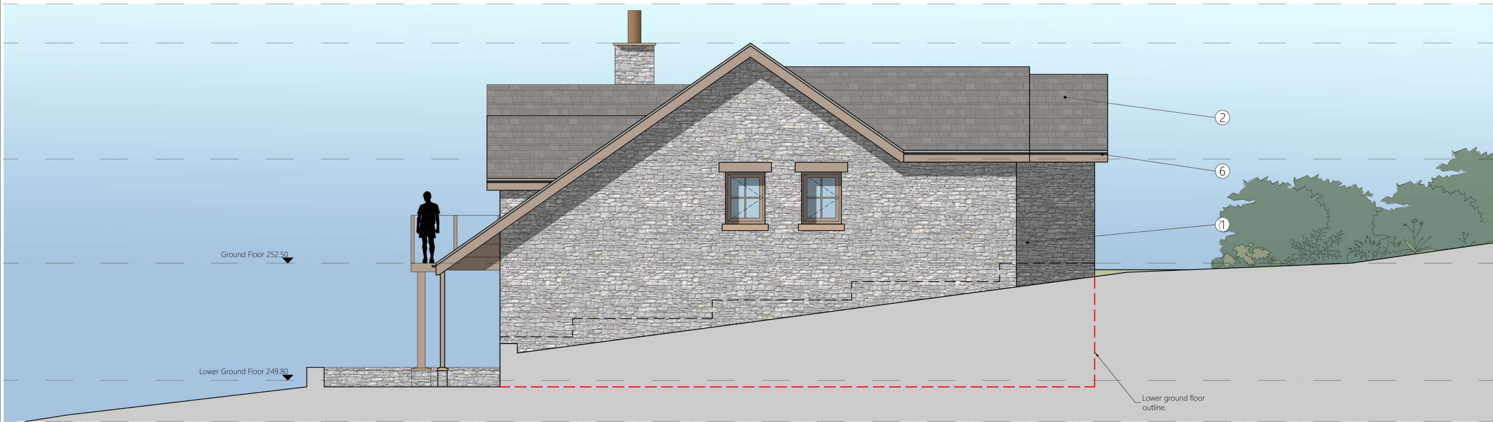
2 Elevation - North 1:50 @ A1 0500
