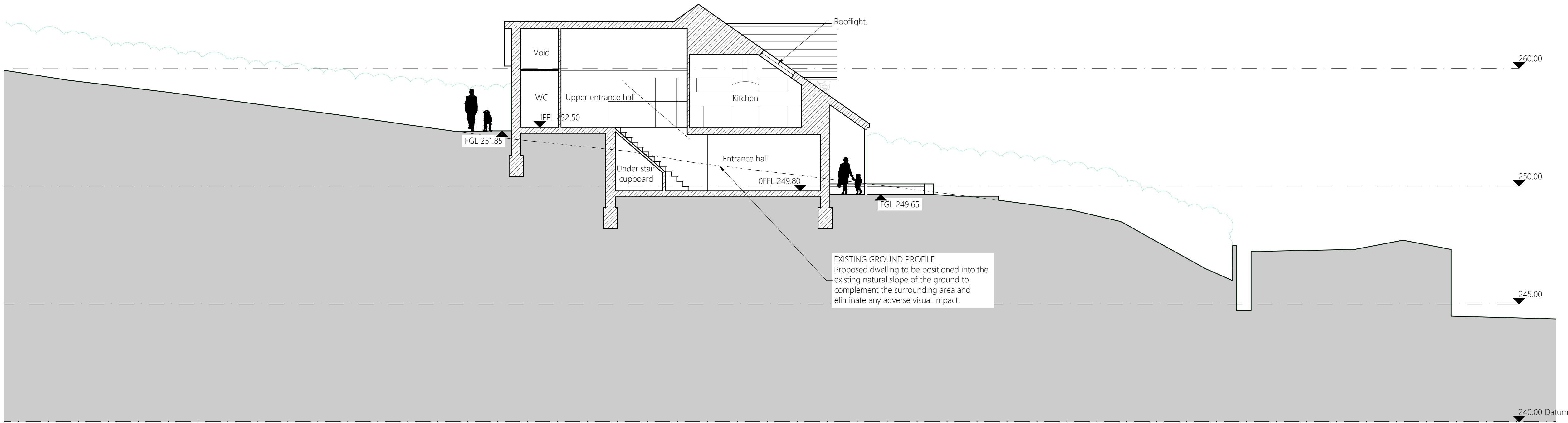
1 Section 1:100 @ A1 Garden Proposed Dwelling Garden Chalets Yard
