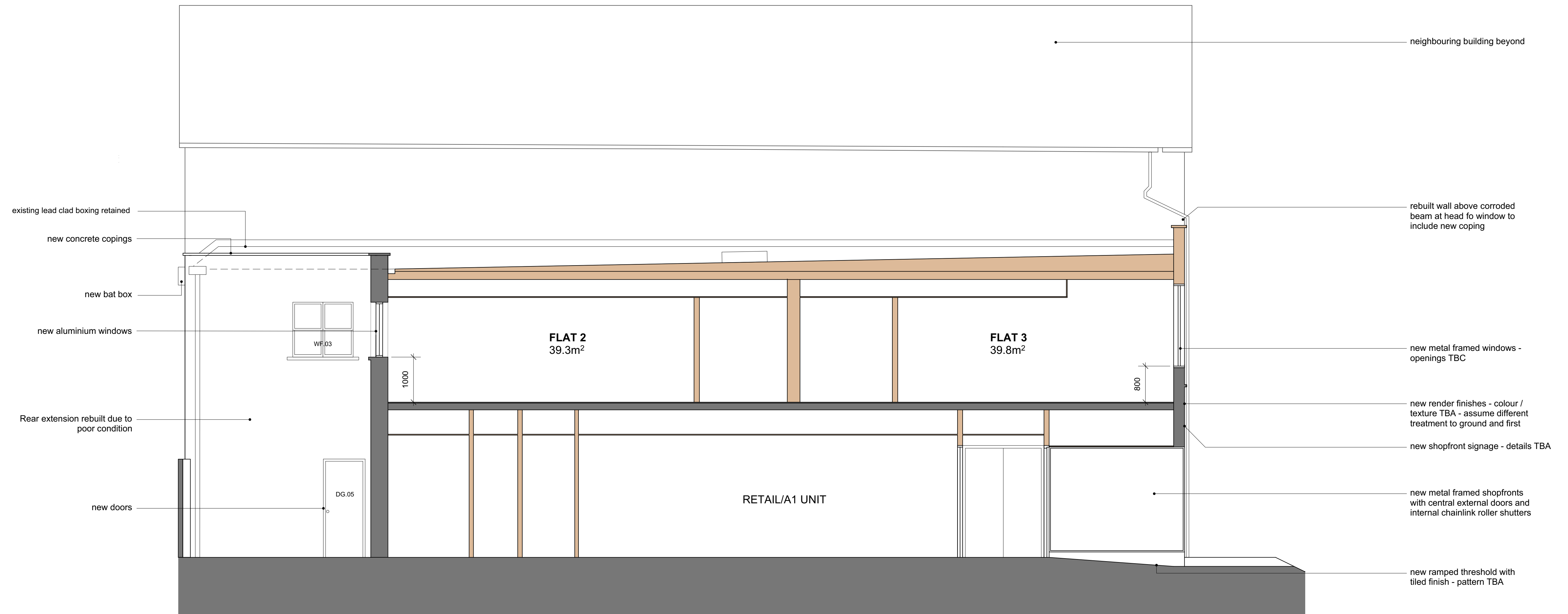
01 proposed section
