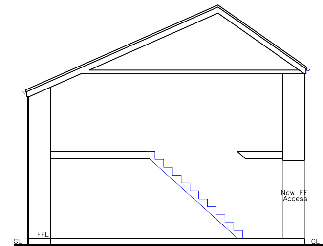
Proposed Section 1:100
