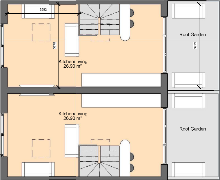
4 Third Floor 1 : 100
