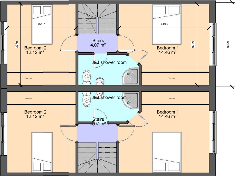
2 First Floor 1 : 100
