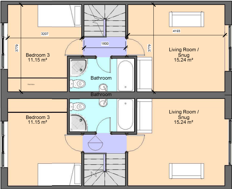
3 Second Floor 1 : 100
