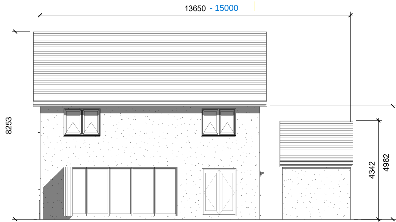
2 Rear Elevation 1 : 100
