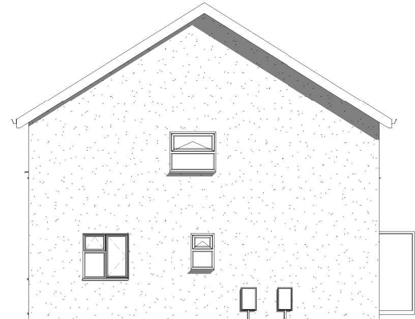
1 Front Elevation 1 : 100
