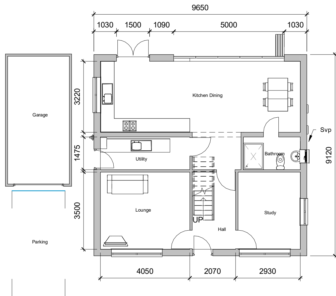
1 Ground Floor 1 : 100
