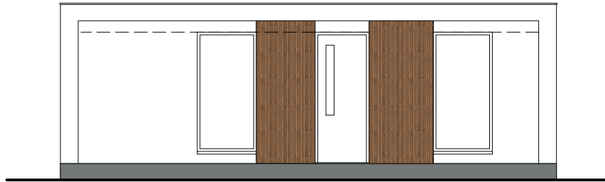
SOUTH/WEST ELEVATION
