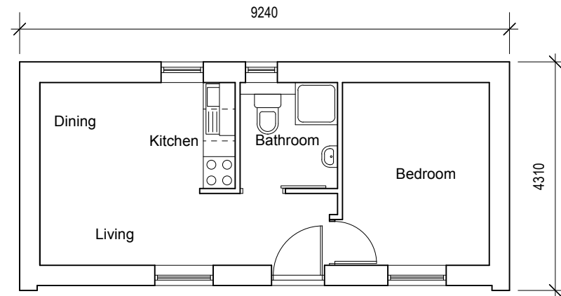
FLOOR PLAN
