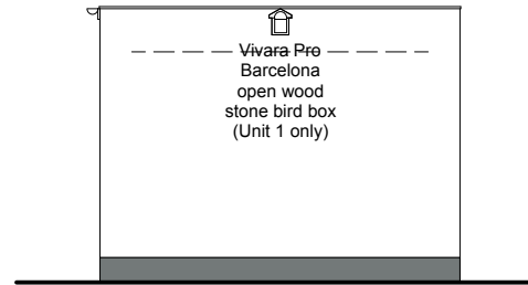
NORTH/WEST ELEVATION
