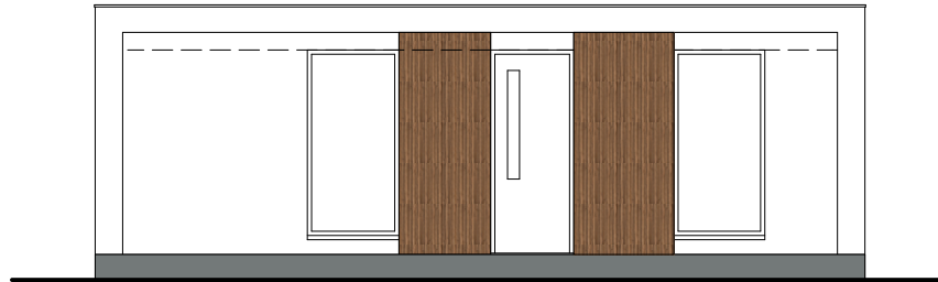
SOUTH/EAST ELEVATION
