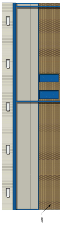
3 Existing Rear Elevation 1 : 100
