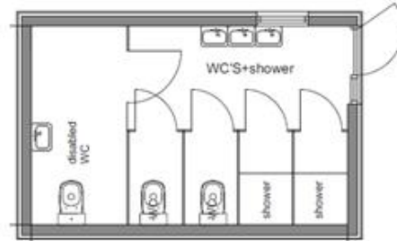
Toilet Block
