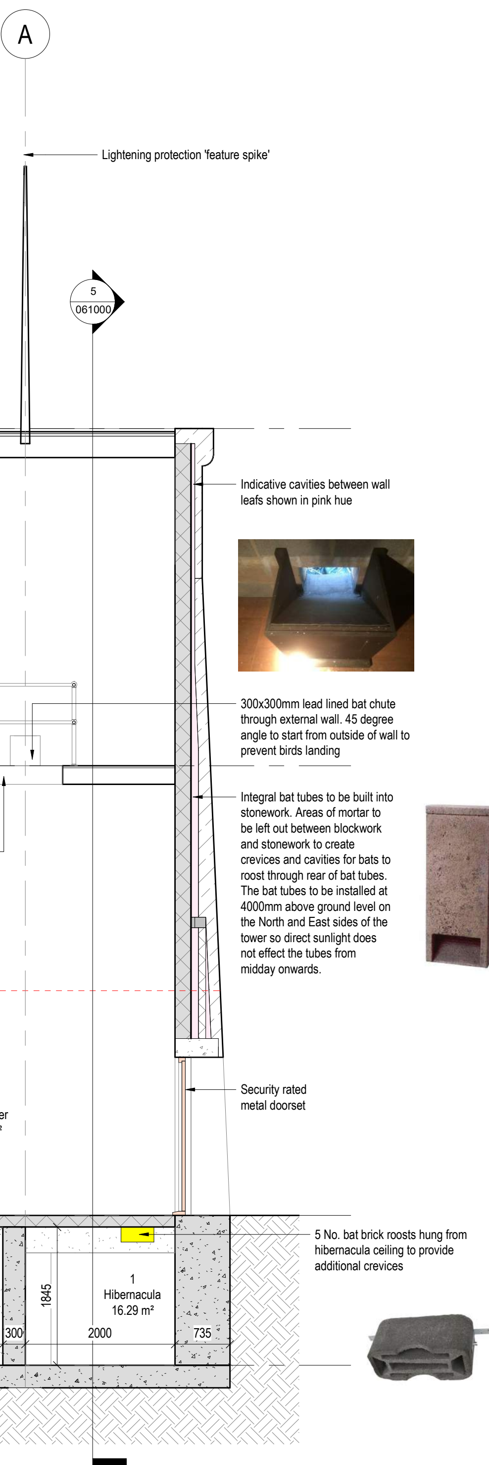
6 | 1 : 50 - GA Section - proposed section W-E
