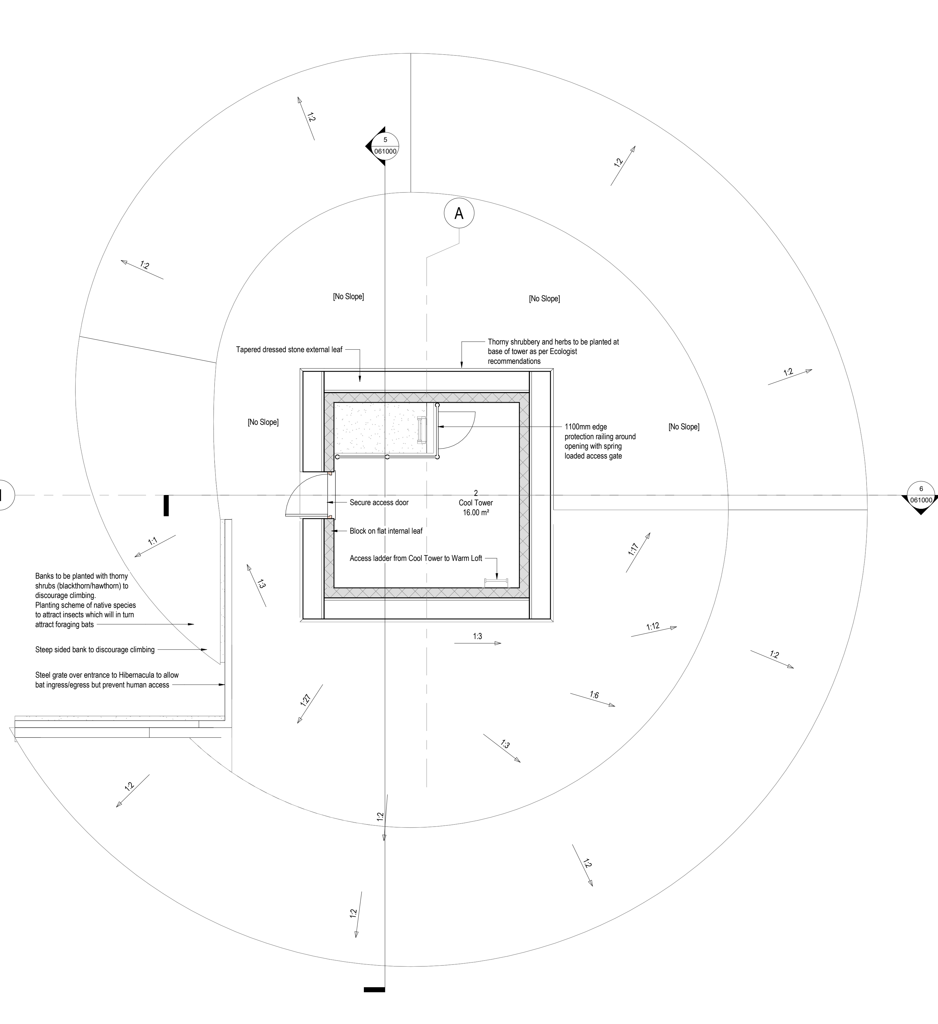
2 | 1 : 50 - GA Plan - 01 - Proposed First Floor Plan
