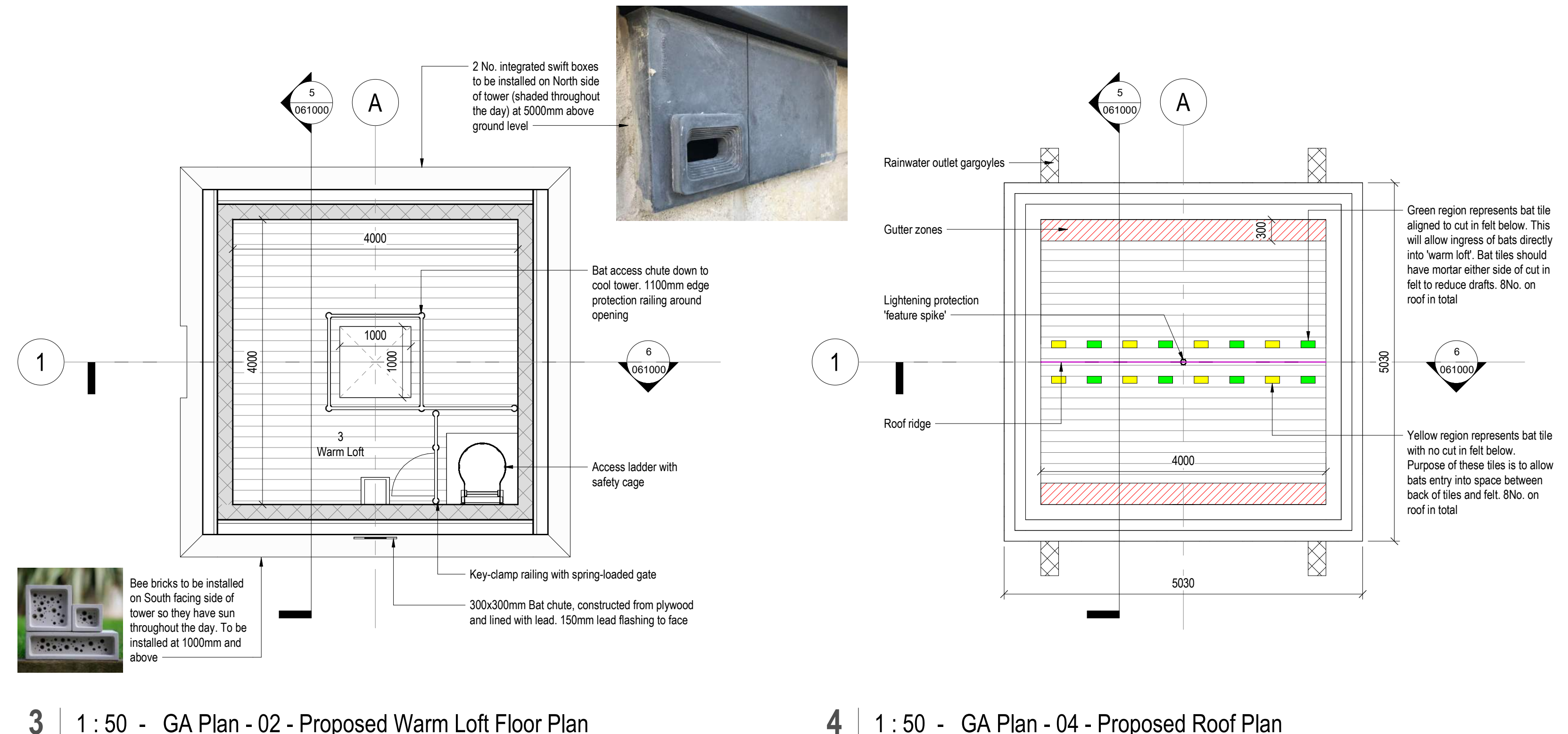
3 | 1 : 50 - GA Plan - 02 - Proposed Warm Loft Floor Plan
