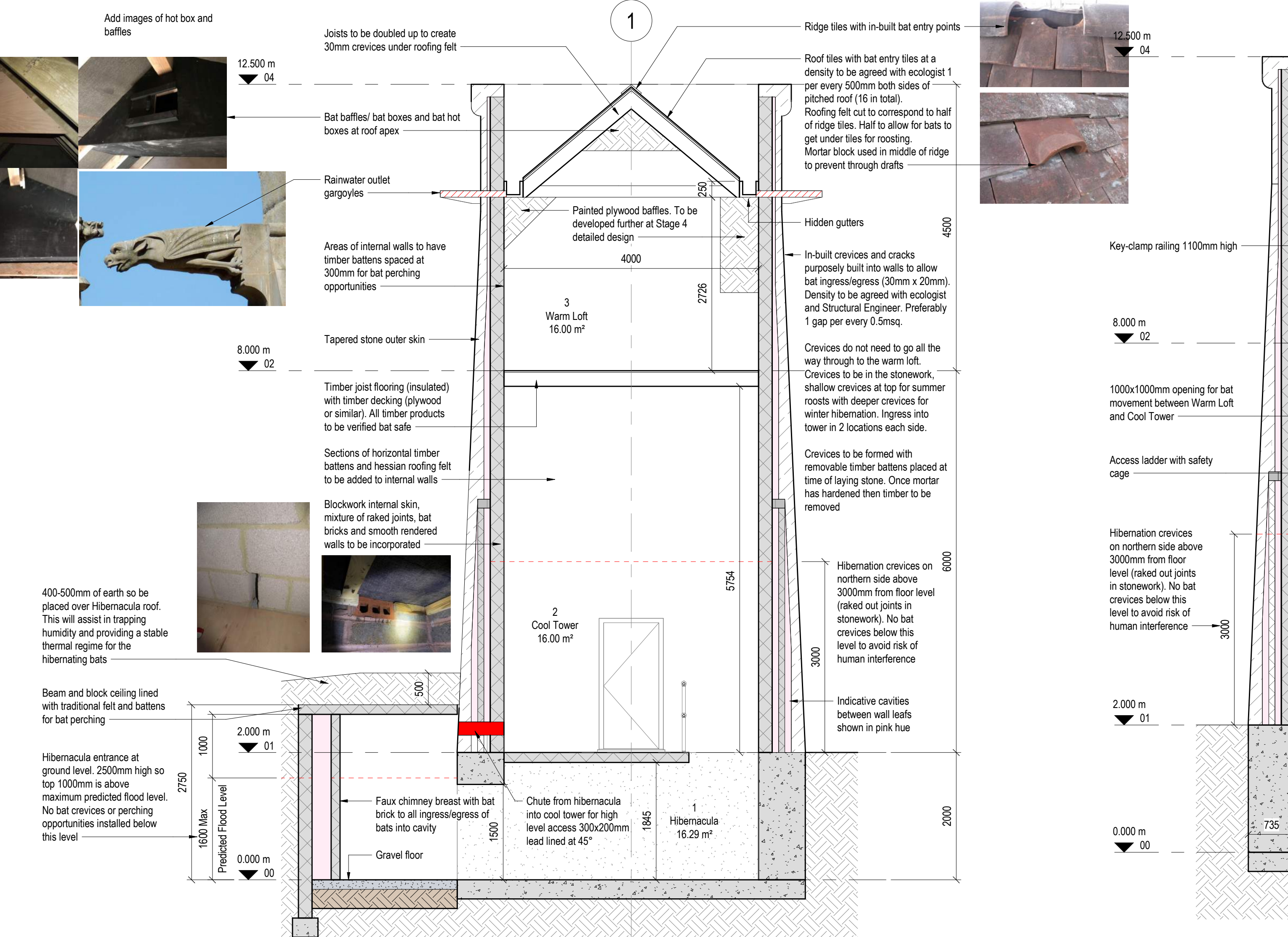
6 | 1 : 50 - GA Section - proposed section W-E
