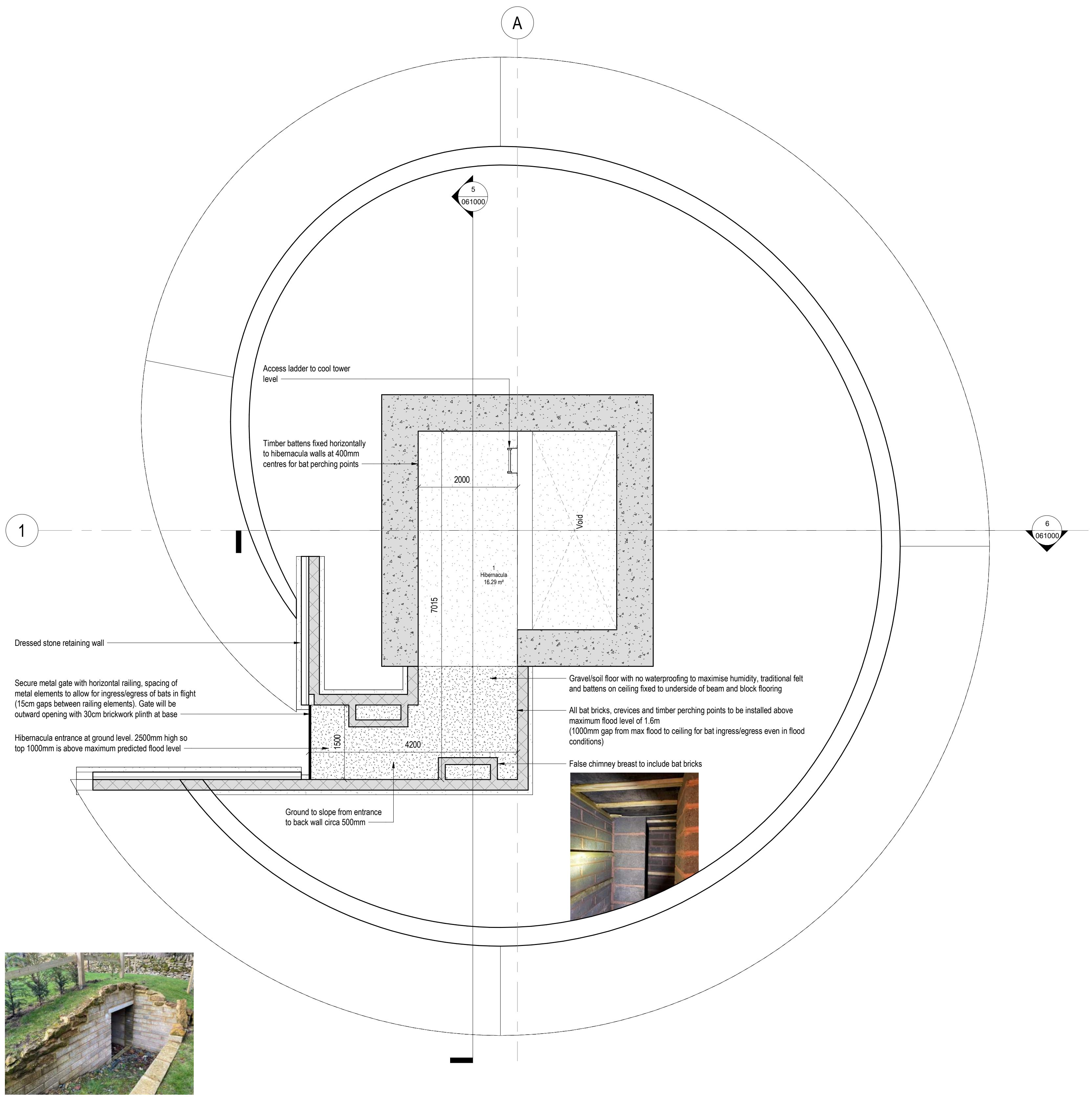
1 | 1 : 50 - GA Plan - 00 - Proposed Hibernacula Floor Plan
