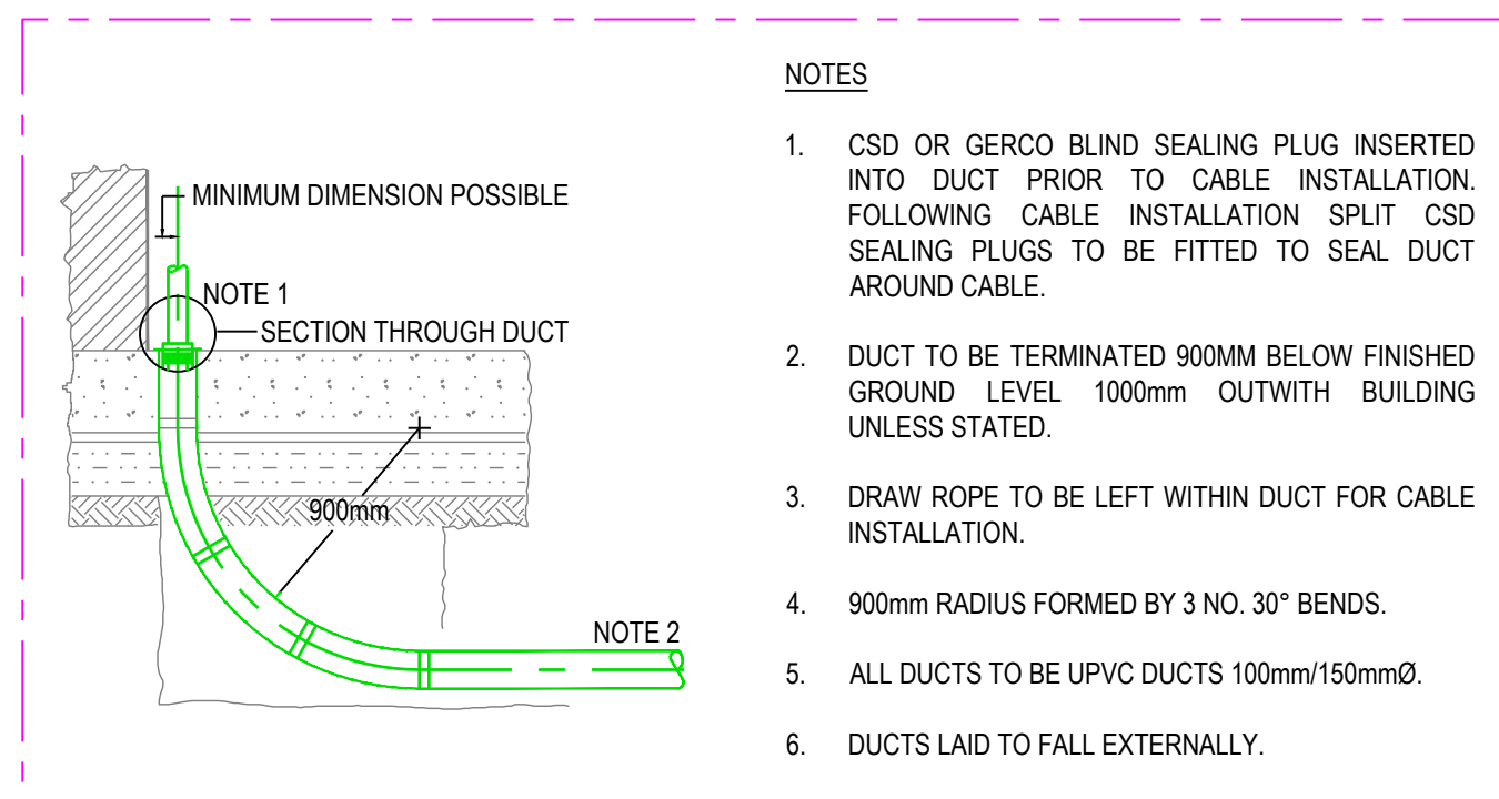
TYPICAL CABLE DUCT ENTRY N.T.S.
