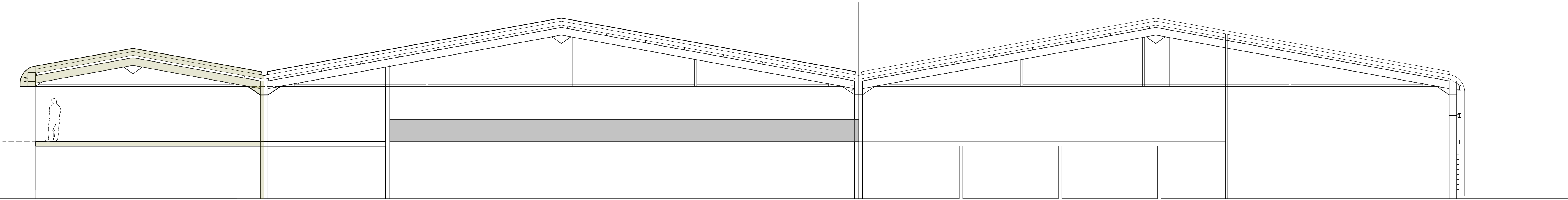
PROPOSED SECTION
