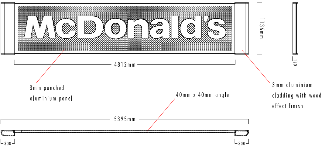
WALL MOUNTED BANNER UNIT scale 1:50
