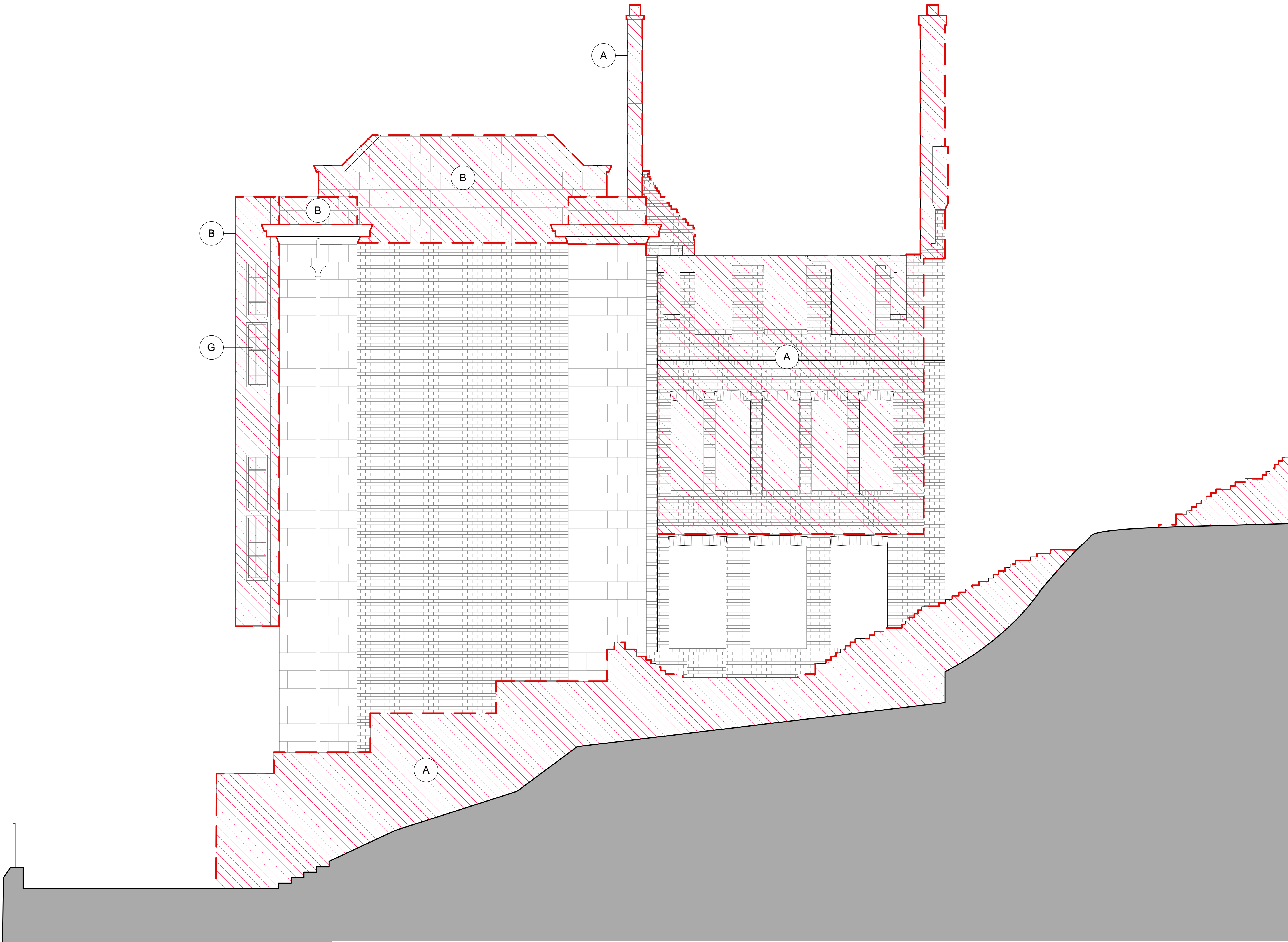
1 East Demolition Elevation Scale: 1:50
