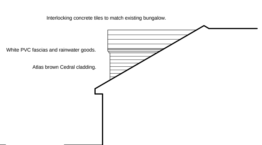
SIDE elevation
