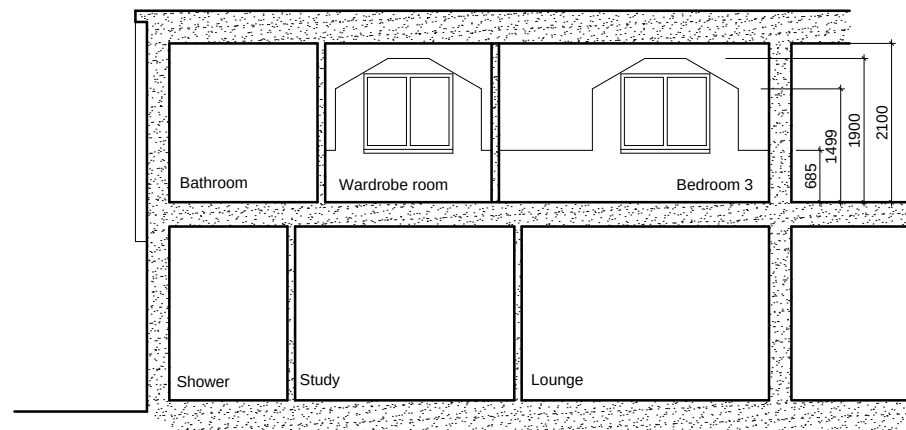
SECTION through Bedroom 3, looking at inside of windows.
