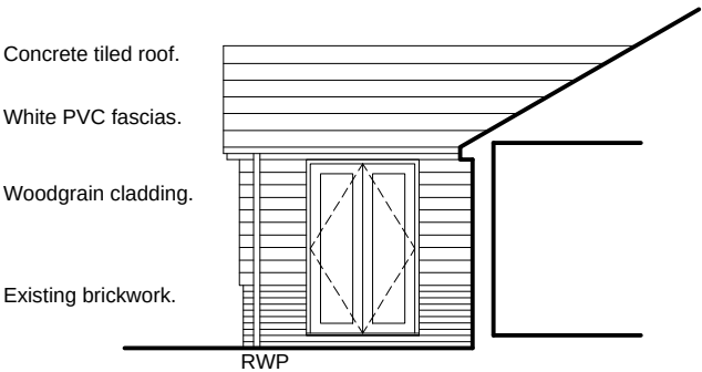
ELEVATION TO GARDEN SIDE
