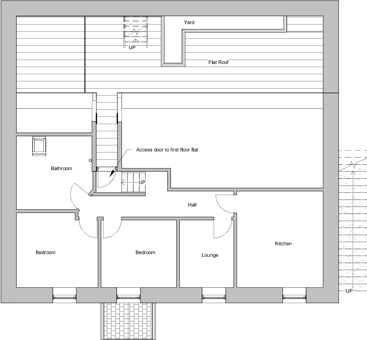
2 Proposed First Floor 1 : 100
